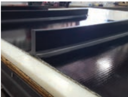
Custom Cleating
